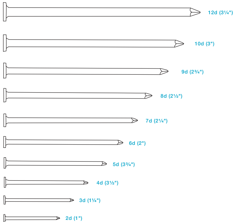
Figure 5: NAIL LENGTHS
