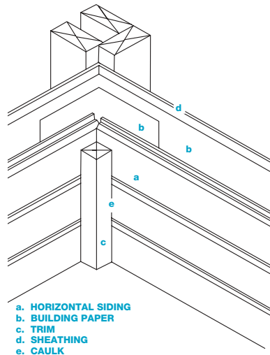
Inside Corner Detail-A
