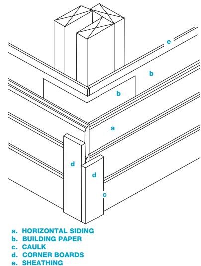
Outside Corner Detail-A
