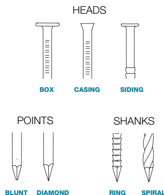
Figure 4: NAIL TYPES
