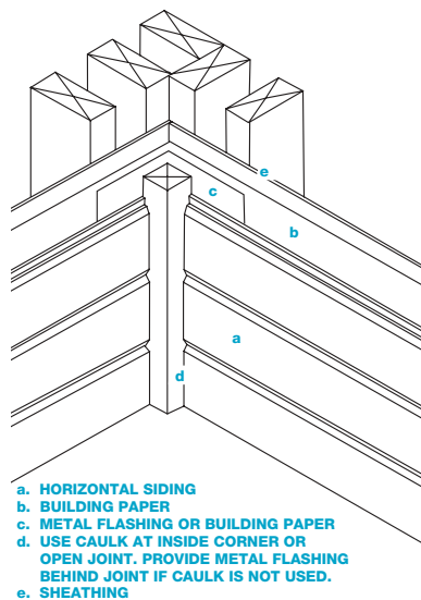
Inside Corner Detail-B
